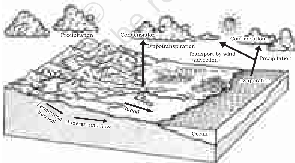
Figure 13.1 : Hydrological Cycle
